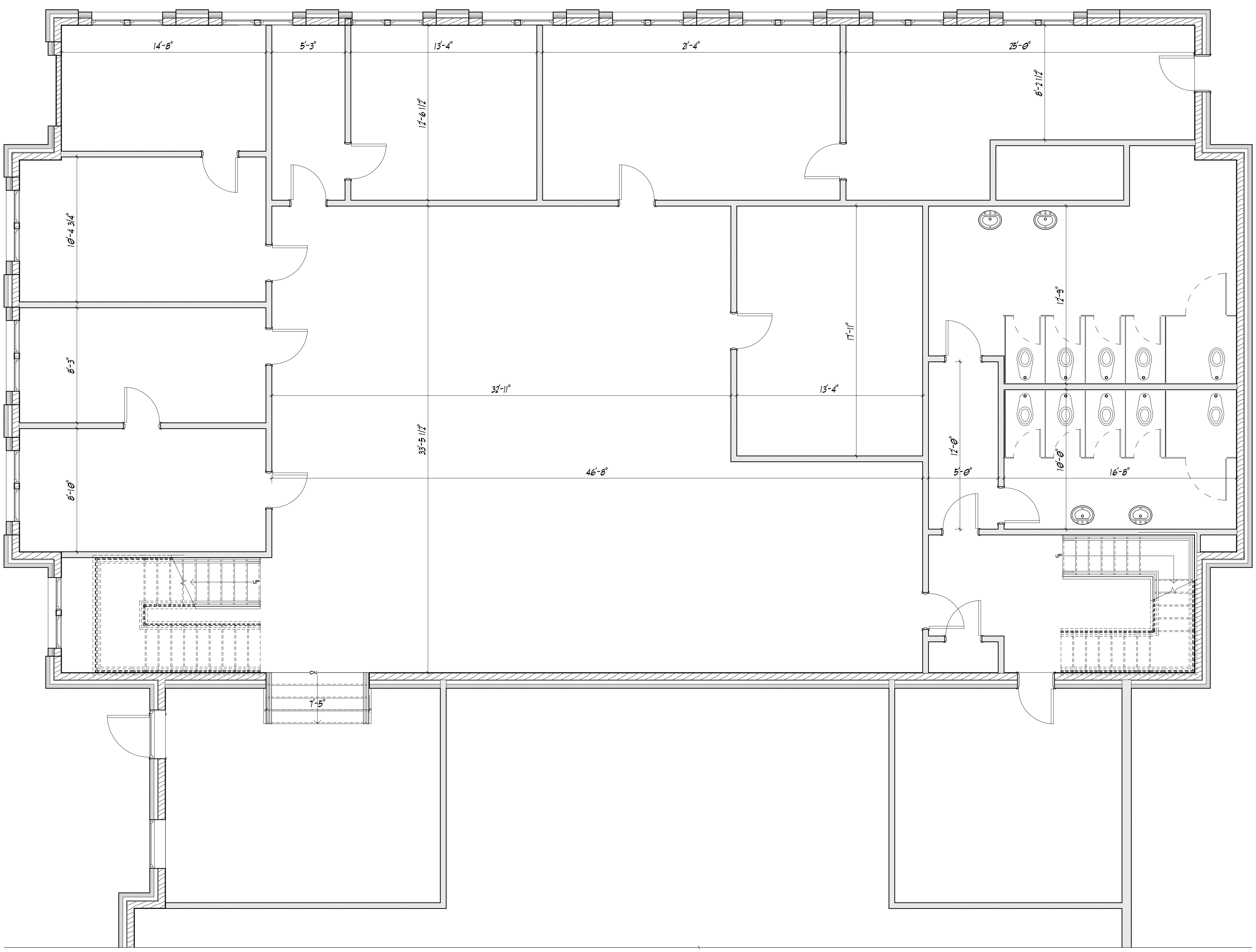
1 EXISTING MAIN LEVEL SCALE: 1/4" = 1'-0"
